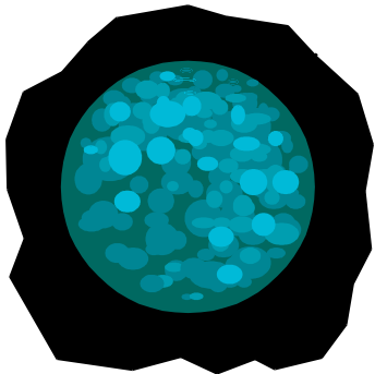
Neptune
