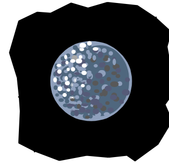
Mercury
